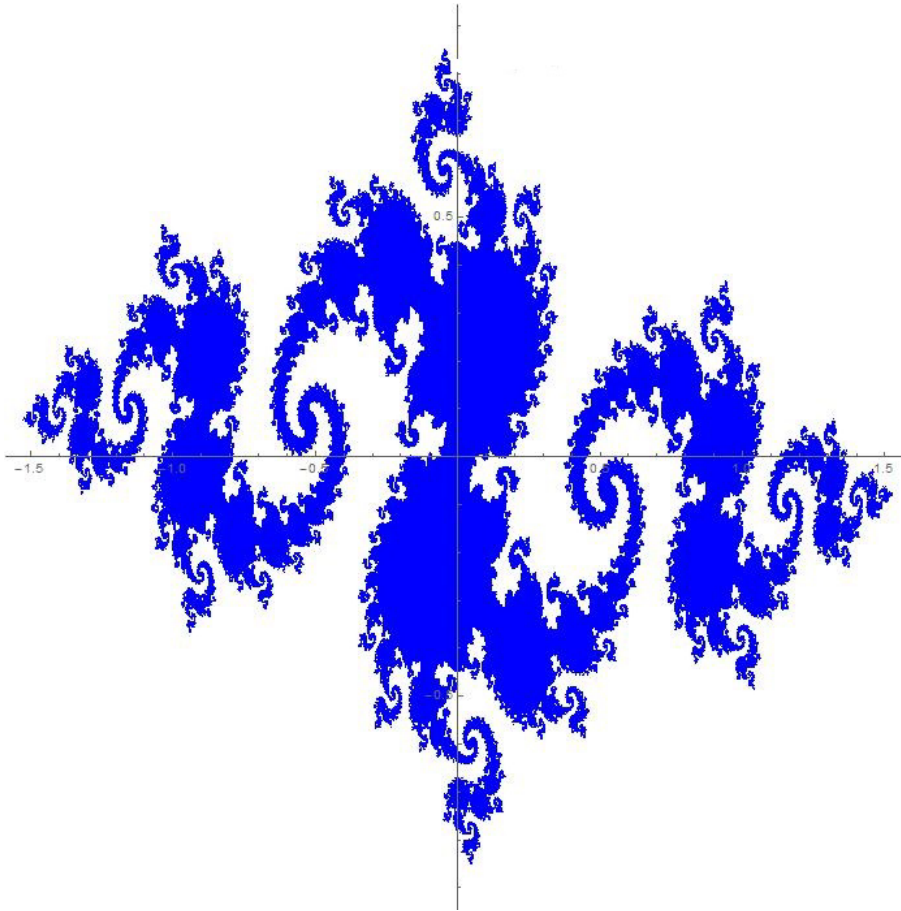
A Julia Set
